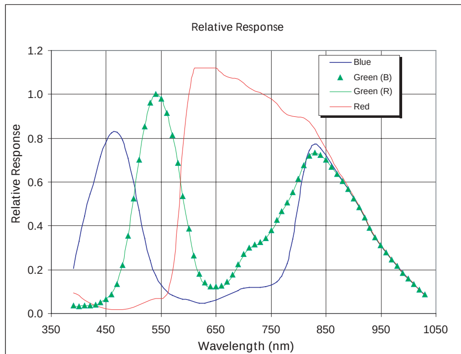
Figure 13: Spectral Response
